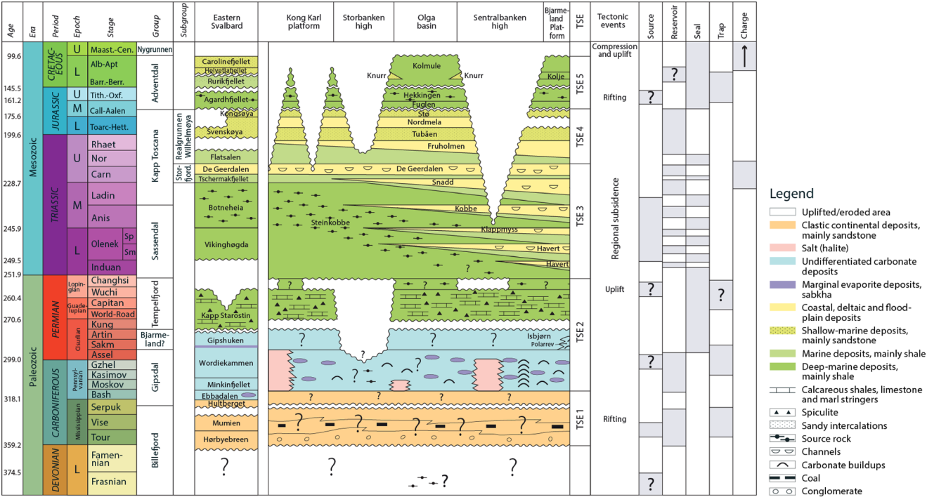
Fig. 4. Tectonostratigraphic chart, orientated SE–NW from the northeastern Bjarmeland Platform to eastern Svalbard, with key geological events. Adapted from NPD (2017). Note that the timescale is non-linear in order to highlight the development of the Triassic succession.
