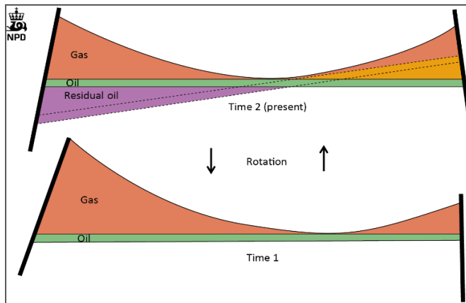
Figure 9 Formation of residual oil zone by rotation of a structural trap with oil and gas. Fluid contacts are controlled by pore pressure and will equilibrate to horizontal surfaces. The pore space where oil is replaced by water will remain with a residual oil saturation (purple zone). There will also be a residual oil saturation in the gas zone (orange zone), but this saturation is much lower than in the water zone. Time 1 – initial trap, Time 2 - rotated trap, dotted lines show the present location of the initial contacts.
