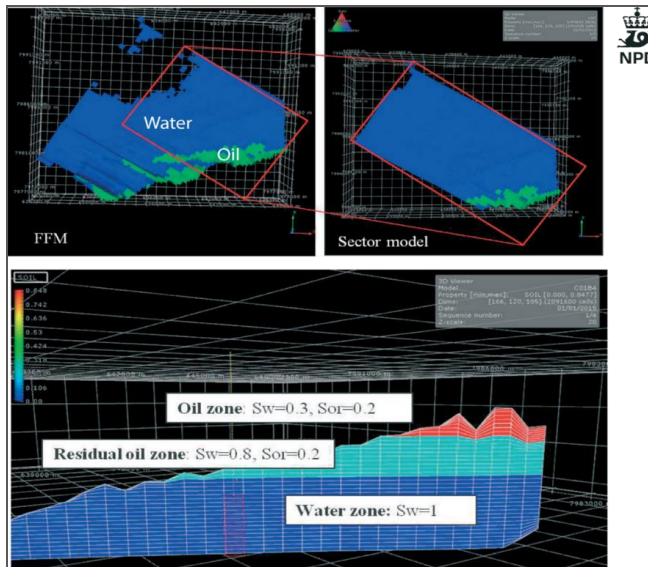
Figure 10 Setup of simulation model, showing the location of the sector model and the distribution of oil and residual oil.
