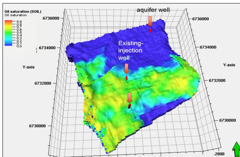
Figure 7 Reservoir model with different location of CO 2 well injection
