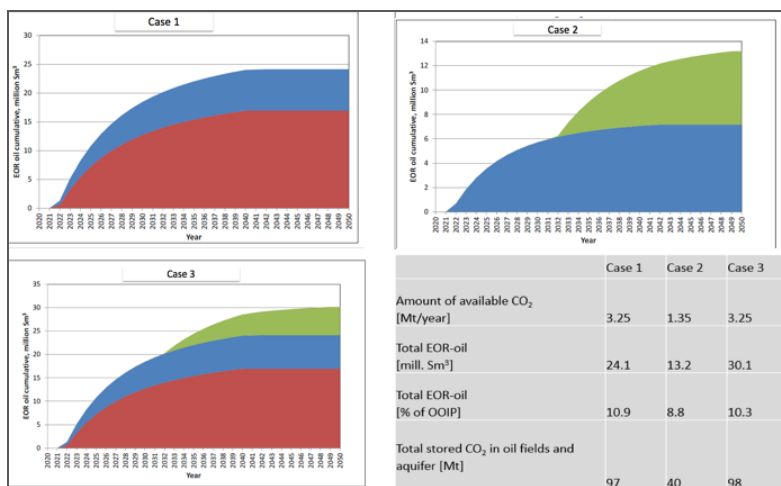
Figure.5 The EOR effect from three oil fields with injection of 1-3 Mt CO 2 annually for EOR and storage, over 30 years.
