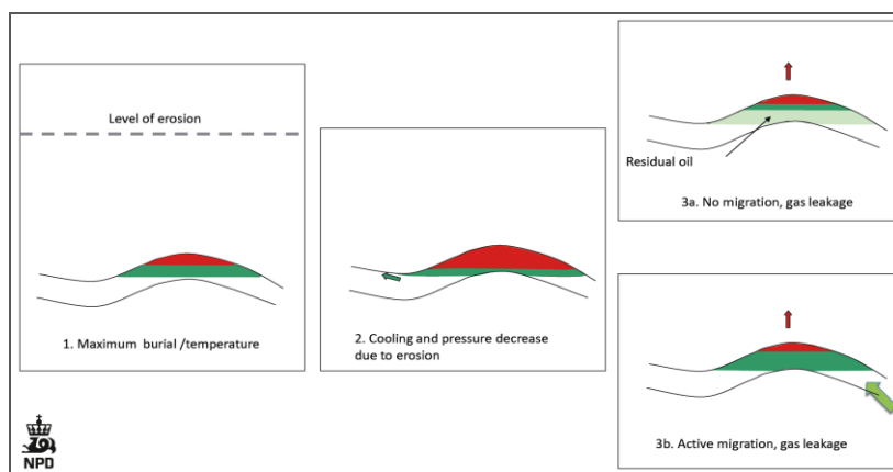
Figure 8 Hypothesis for formation of residual oil zone by natural gas seepage. After maximum burial the rate of seepage of gas is greater than the rate of migration of hydrocarbons into the accumulation. Consequently, fluid contacts move upwards. Residual oil (light green) is formed where water replaces oil in the initial oil zone (green).
