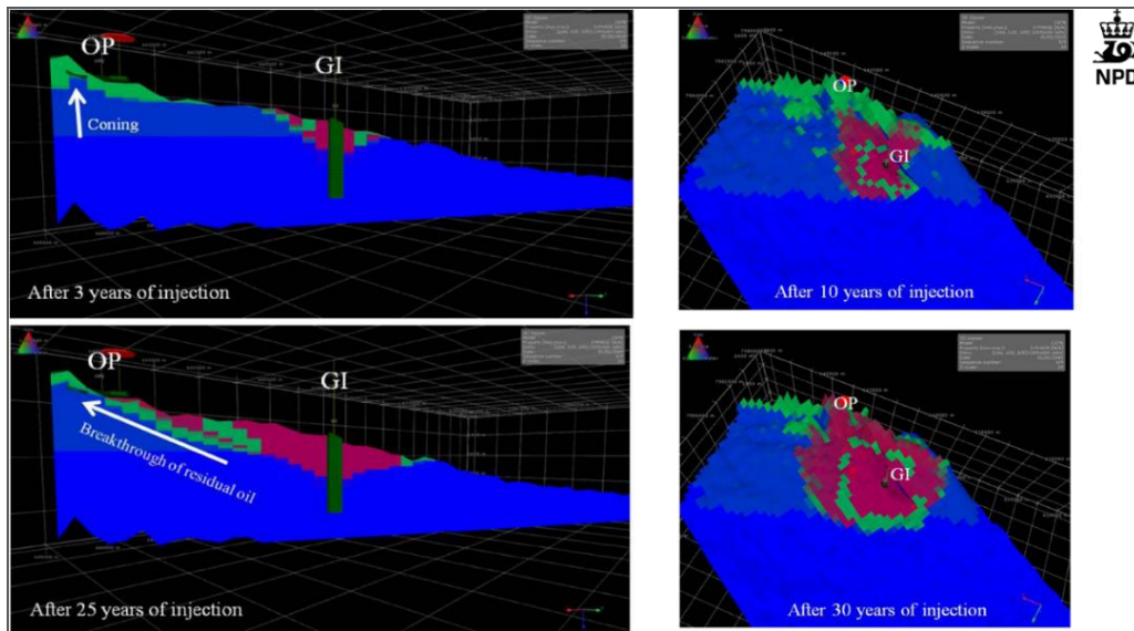
Figure.11 Profiles through the CO 2 injector (GI) and the oil producer (OP), showing distribution of CO 2 (red), oil (green) and water (blue) 3 and 25 years after the injection start. The maps to the right show the distribution of the CO 2 plume. North is down to the left.
