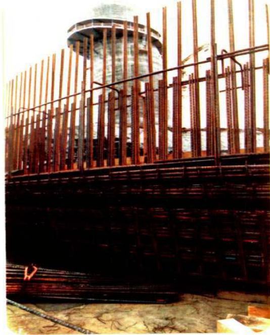
Figure 8 Reinforcement [13].
