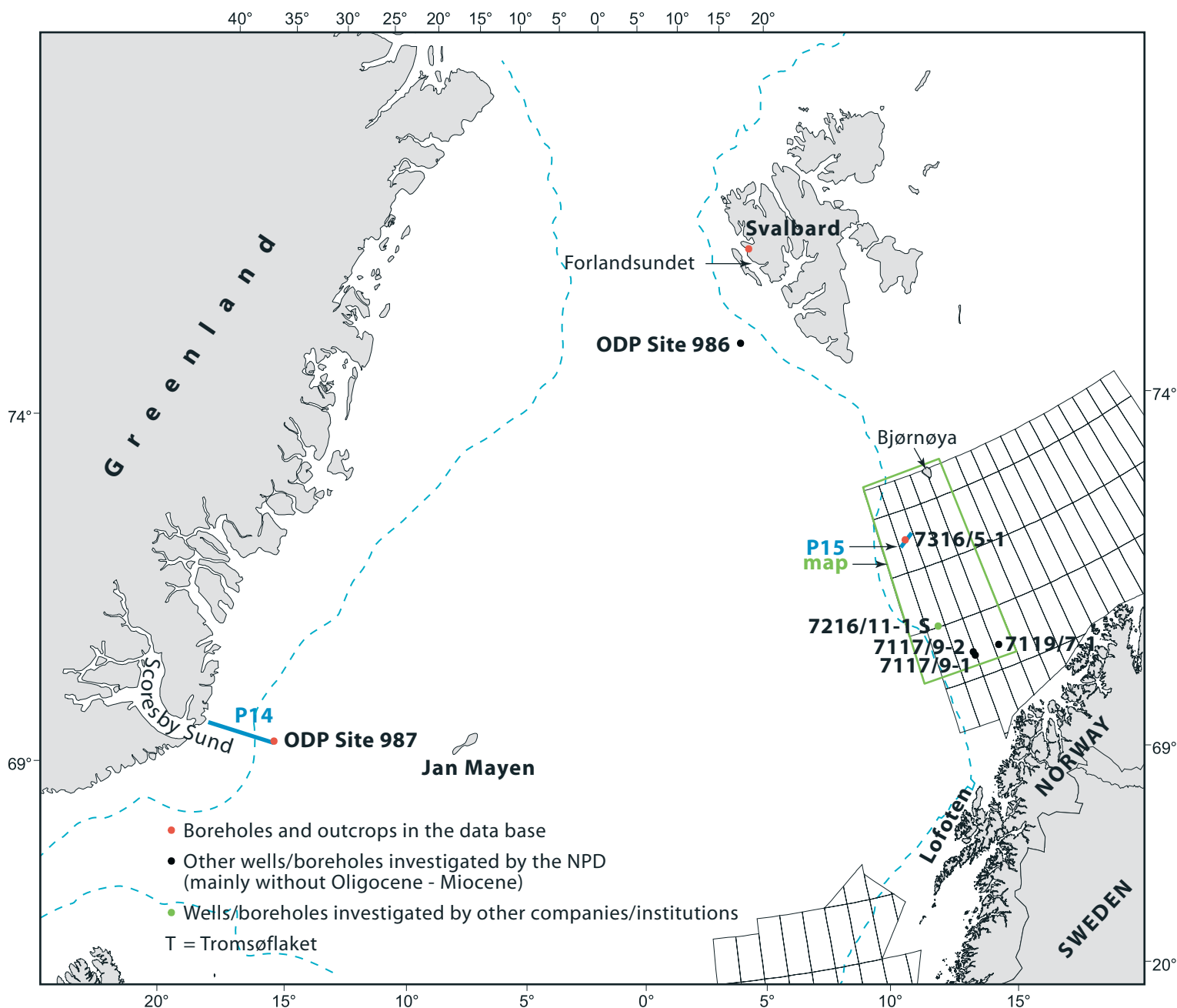
Map 2: Oligocene to Lower Pliocene well, borehole and outcrop database and seismic profiles in the western Barents Sea, Svalbard and East Greenland (off Scoresby Sund).
