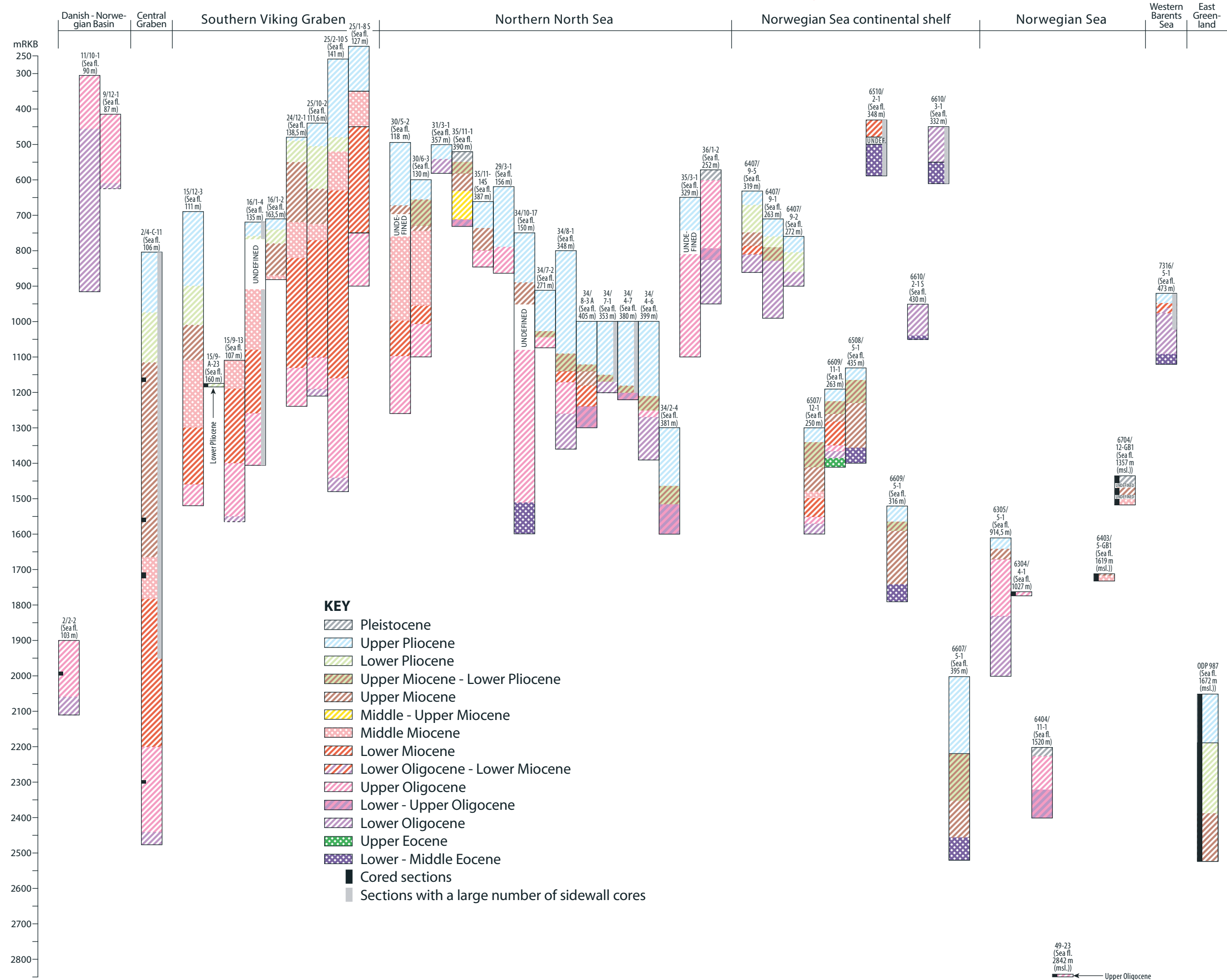
Diagram/Fig. 2: Chronostratigraphy of studied wells and boreholes. All depths are in metres below rig floor, except for the boreholes 6704/12-GB1 and 6403/5-GB1 and the core 49-23 which are in metres below mean sea level. The onshore Hjøllund and Rødding boreholes and the outcrop at Sarsbukta (Forlandsundet, Spitsbergen) in figure 1 are not included in this figure.
